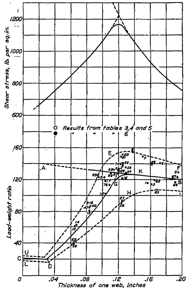
FIGURE 1.—The relation between load-weight ratio and thickness of web for 3 by 8 1/4 inch box beams with the grain of the plywood webs at ±45 degrees to the length of the beam. Flange depth 1 1/4 inches
